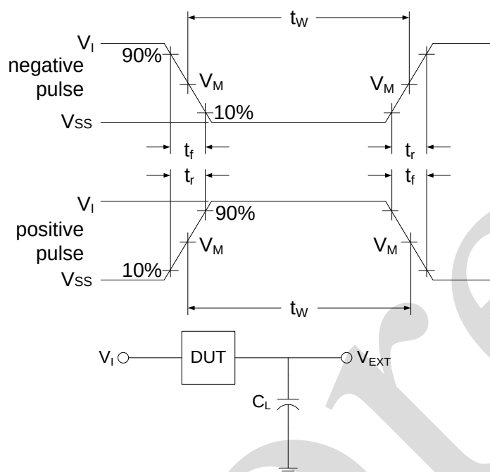
Figure 3. Load circuit
