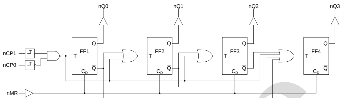
Figure 1. Functional diagram
