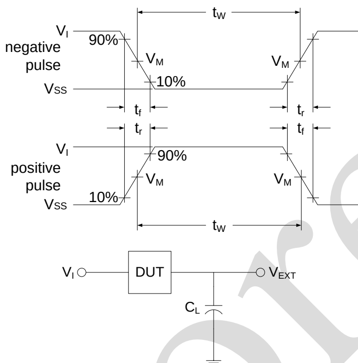
Figure 3. Load circuit
