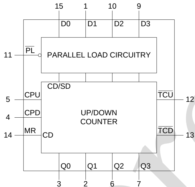
Figure 1. Functional diagram
