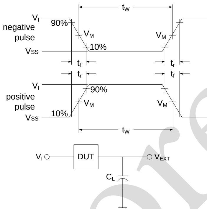
Figure 3. Load circuit
