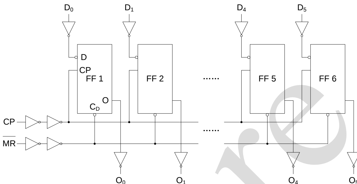
Figure 1. Functional diagram
