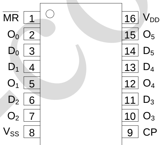
Figure 2. Pin configurations
