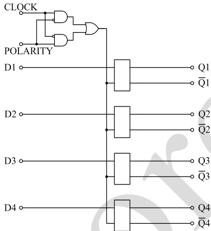
Figure 1. Functional diagram
