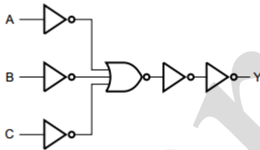
Figure 2. Logic diagram
