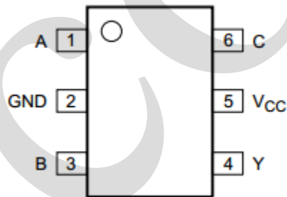
Figure 3. Pin configurations
