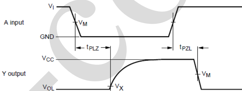
Figure 4. The input A to output Y propagation delays
