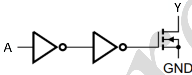
Figure 2. Logic diagram (one gate)
