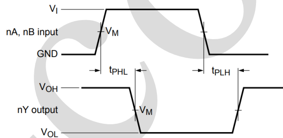
Figure 4. The data input (A, B) to output (Y) propagation delays
